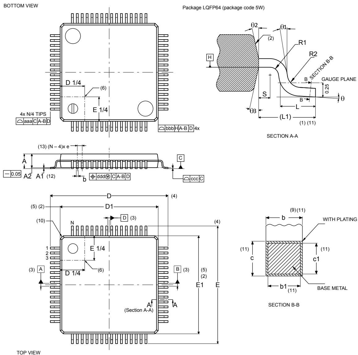
Figure 82. LQFP64 - Outline (15.)
