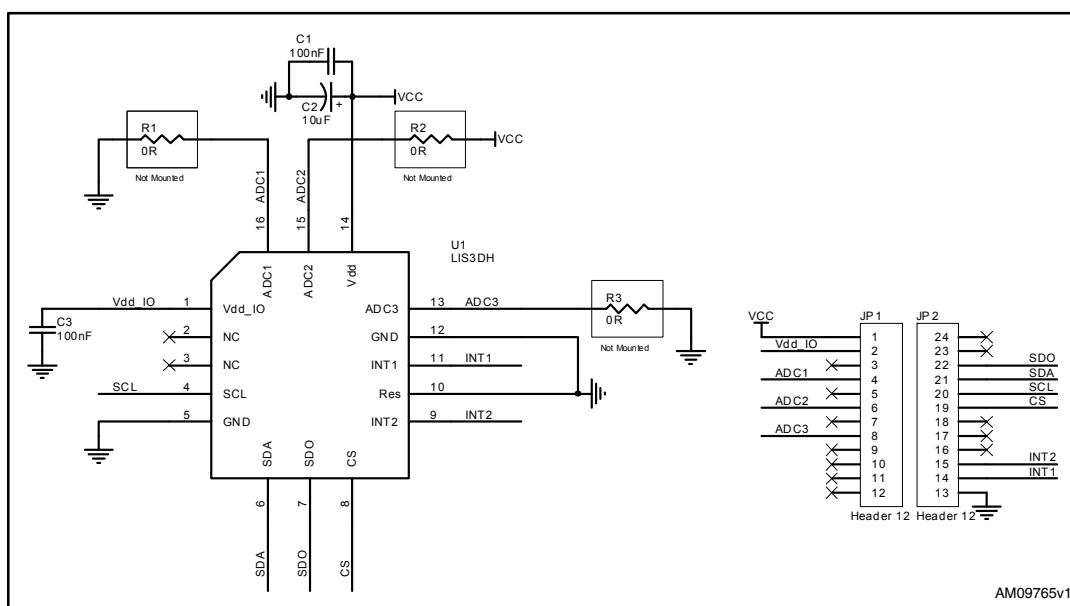
Figure 1: STEVAL-MKI105V1 circuit schematic
