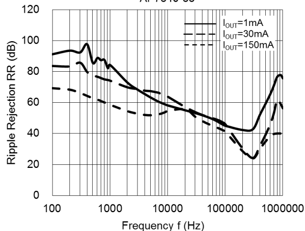
Ripple Rejection vs. Frequency AP7340-33
