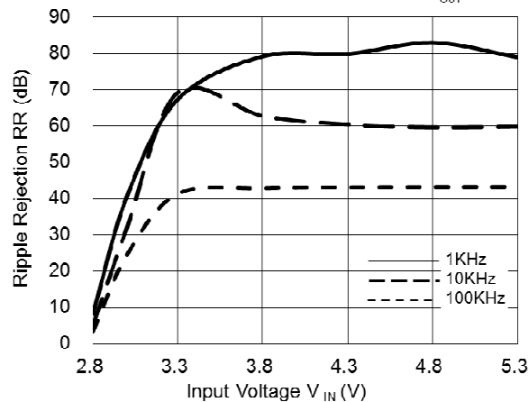
Ripple Rejection vs. Input Bias Voltage AP7340-28 I_{OUT}=30mA
