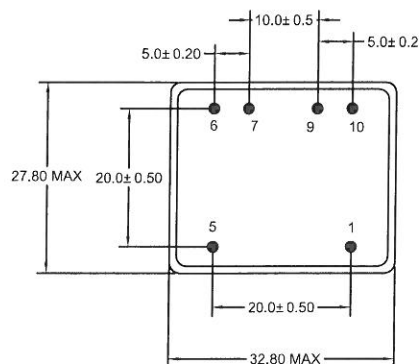
Dual outputs
