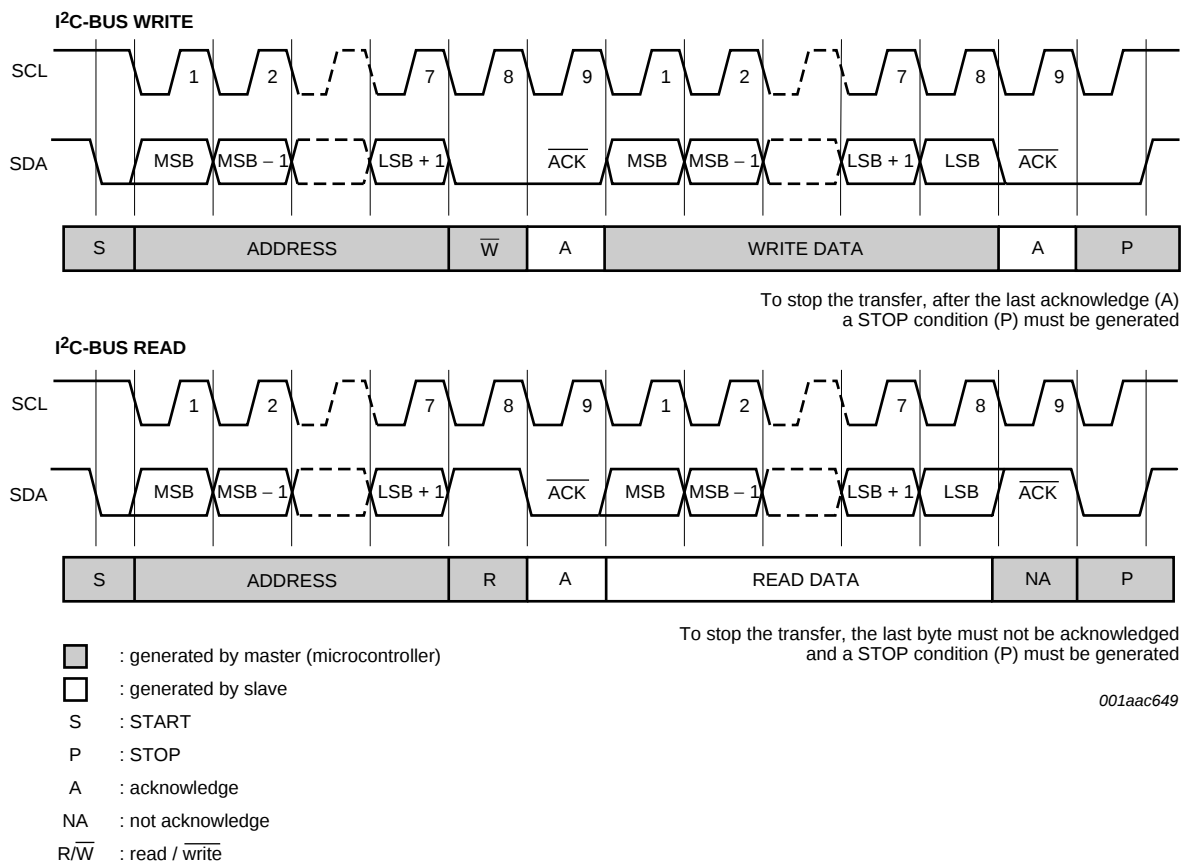
Fig 17. I 2 C-bus read and write modes
