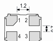
Underside View
