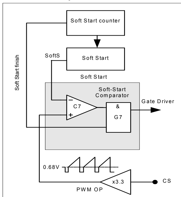
Figure 9 Soft Start
