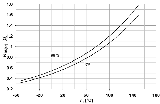
Figure 63 Drain-source on-state resistance; R_{DS(on)} = f(T_J) ; I_D = 4.5A ; V_{CC} > 10.5V
