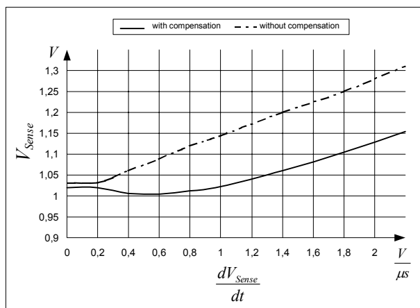
Figure 20 Overcurrent Shutdown
