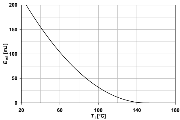
Figure 64 Avalanche energy; E_{AS} = f(T_J) , I_D = 3A , V_{DD} = 50V
