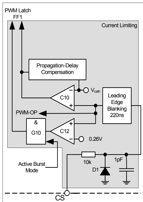
Figure 17 Current Limiting Block
