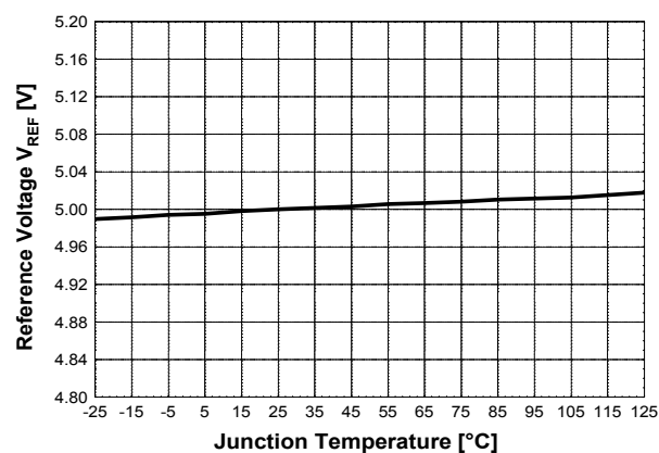
Figure 37 Reference Voltage V_{REF}
