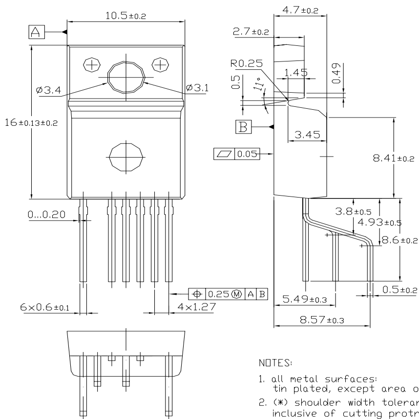
Figure 70 PG-TO220-6-347 (PB-free Plating Fullpak Package)
