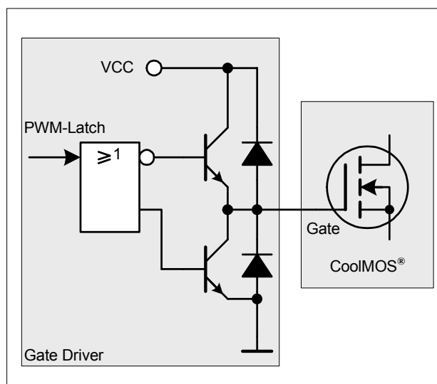
Figure 15 Gate Driver
