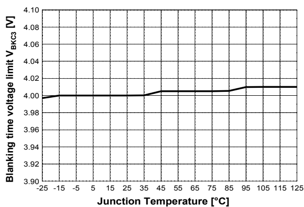
Figure 45 Blanking time voltage limit V_{BK3}
