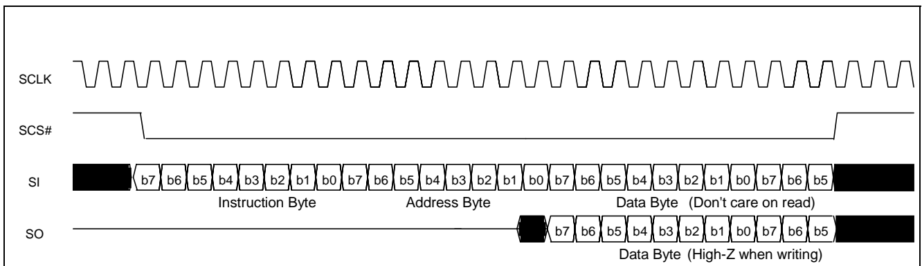
SPI Slave Mode Timing
