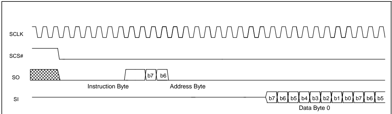
SPI Master Mode Timing
