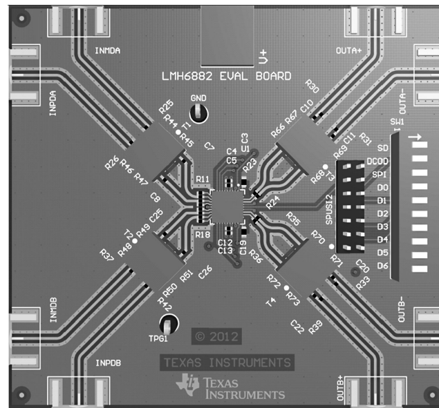
FIGURE 1. LMH6882EVAL
