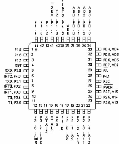
44-Pin QFP
