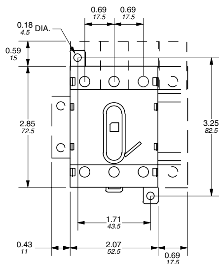
CDNF30, CDF60, CDF100 — base & DIN rail mounted switch
