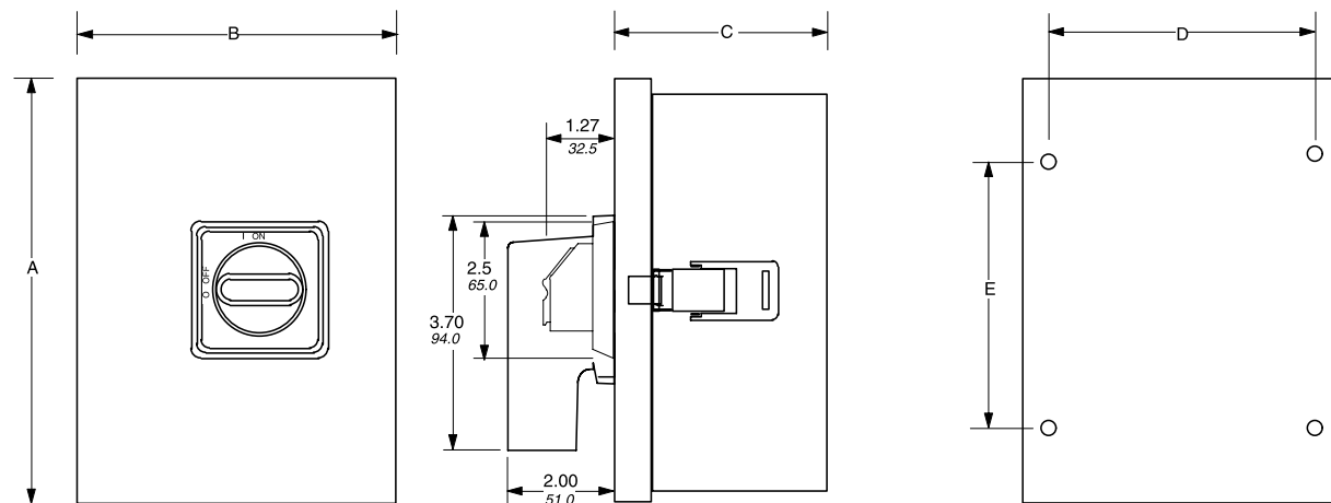
Type 1 — 2, 3 & 4 Pole non-fusible switches
