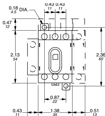
CDNF16, CDF25, CDF32 — base & DIN rail mounted switch
