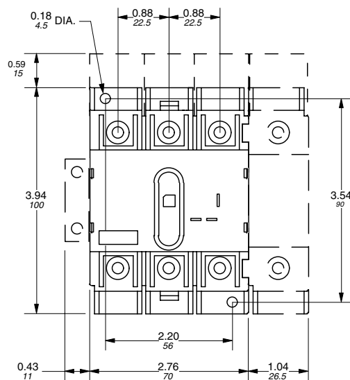
CDNF30, CDF60, CDF100 — base & DIN rail mounted switch
