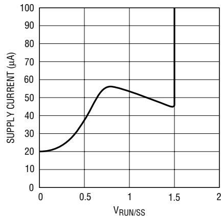
Supply Current in Shutdown vs V_{RUN/SS}
