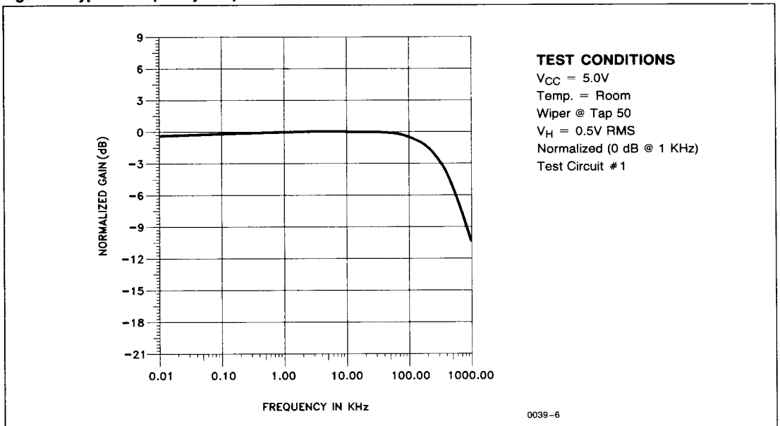
Figure 4: Typical Frequency Response for X9103
