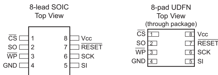
Figure 1-1. Pinouts
