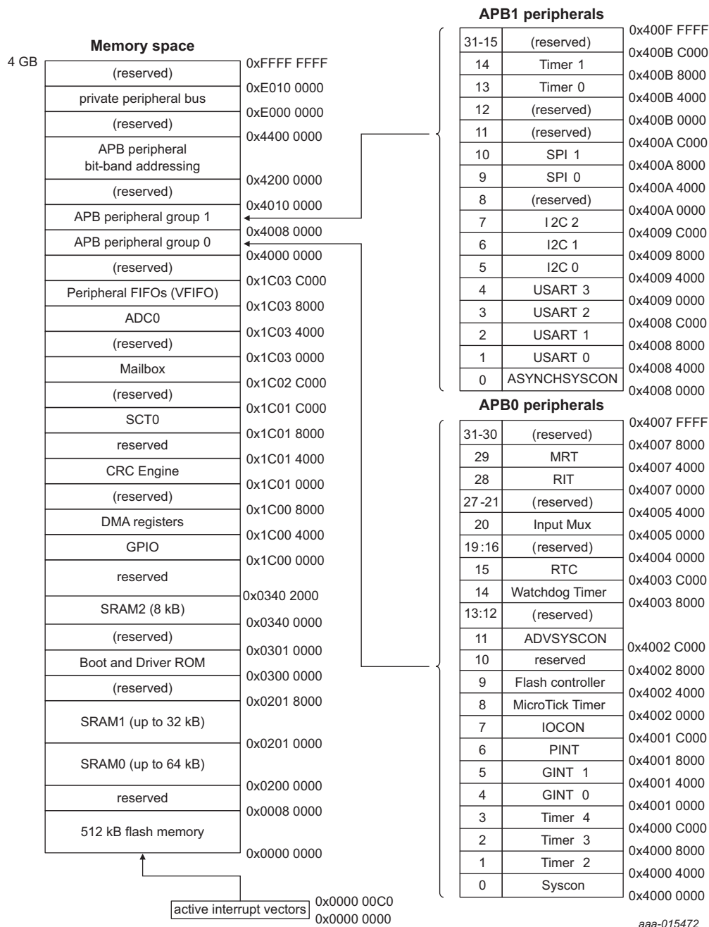
Fig 6. LPC5410x Memory mapping
