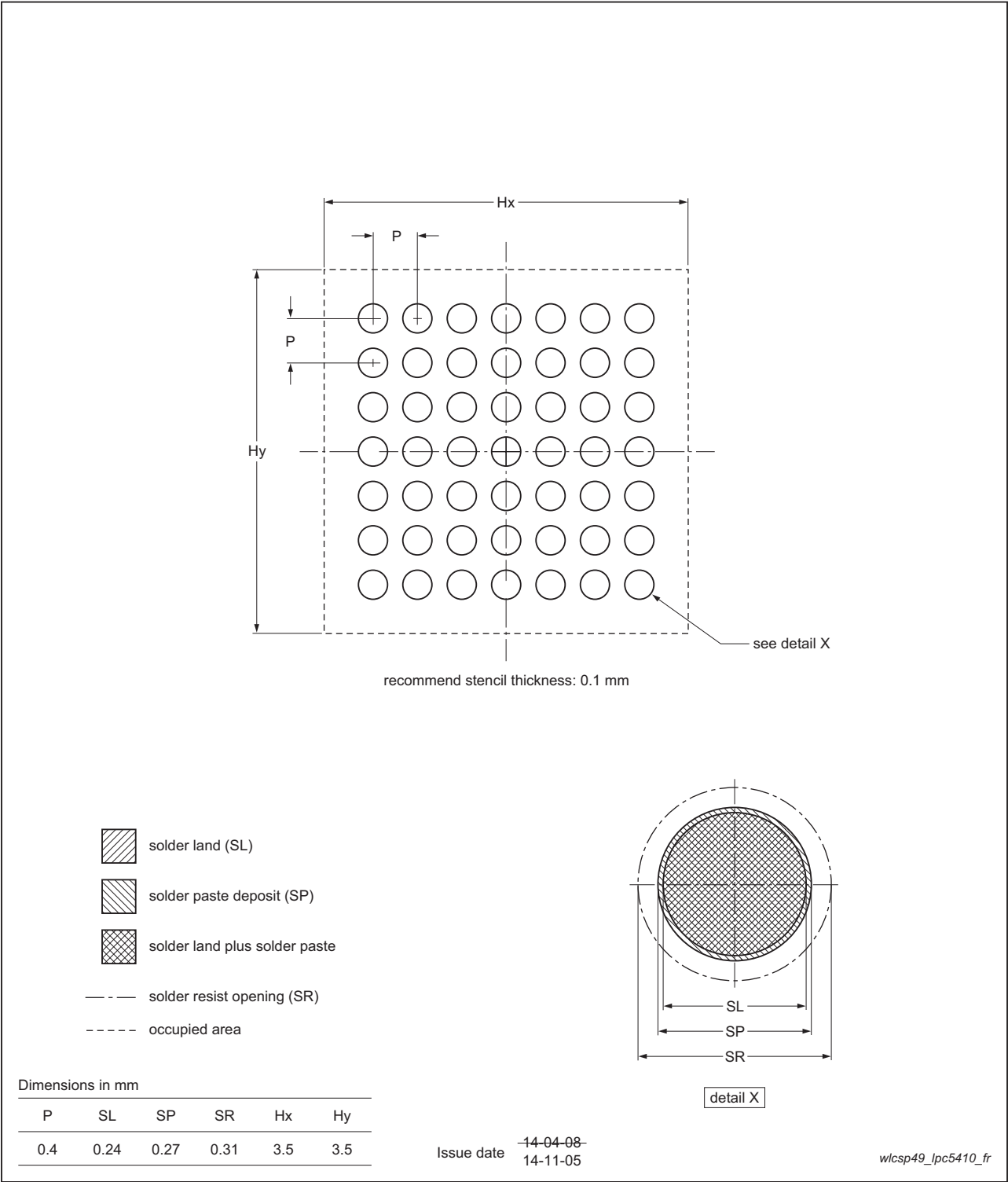
Footprint information for reflow soldering of WLCSP49 package
