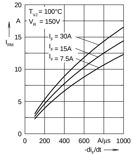
Fig. 3 Peak reverse current I_{RM}
