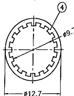
RECOMMENDED MOUNTING HOLE (建議安裝孔)
