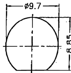
RECOMMENDED MOUNTING HOLE (建議安裝孔)
