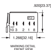
VC2 CONNECTOR HOUSING (For AMP terminals only)
