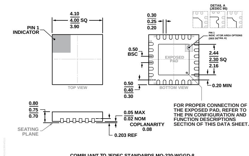
Figure 34. 24-Lead Lead Frame Chip Scale Package [LFCSP] 4 mm × 4 mm Body and 0.75 mm Package Height (CP-24-14)
