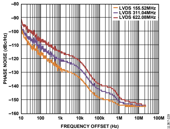
Figure 27. Absolute Phase Noise in LVDS Mode with Clock Input at 622.08 MHz and Outputs = 622.08 MHz, 311.04 MHz, and 155.52 MHz
