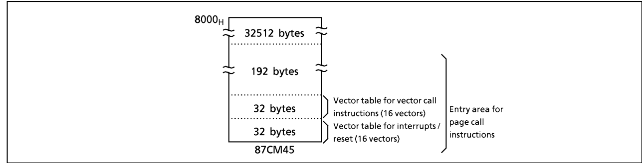
Figure 1-2. ROM Address Maps
