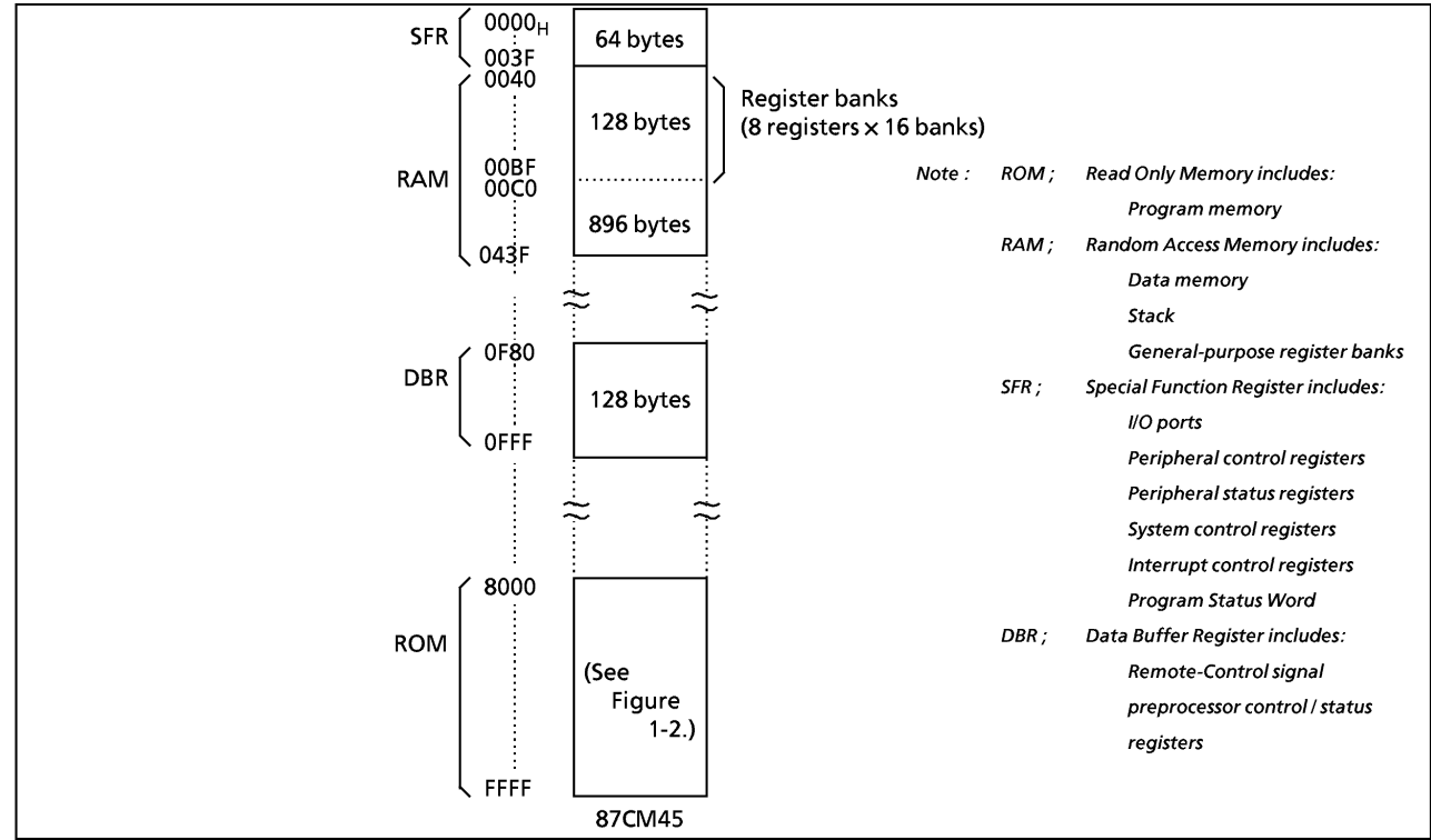
Figure 1-1. Memory Address Map
