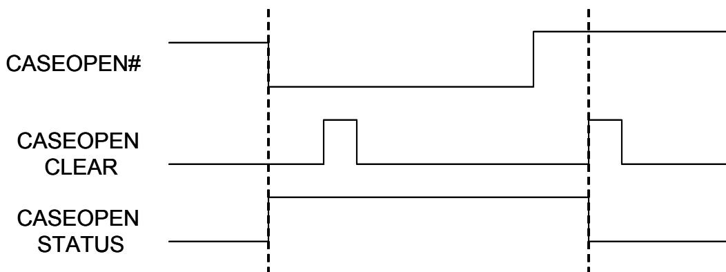
Figure 8-24 Caseopen Mechanism
