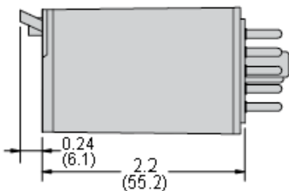
Full Featured Dimensions
