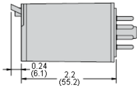
Full Featured Dimensions
