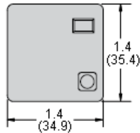
Plain Cover Dimensions
