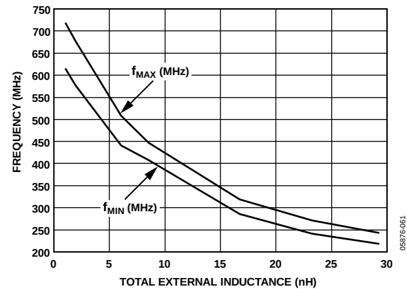
Figure 37. Direct RF Output vs. Total External Inductance
