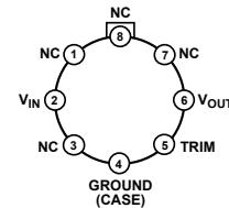
Figure 1. TO-99 (J-Suffix)
