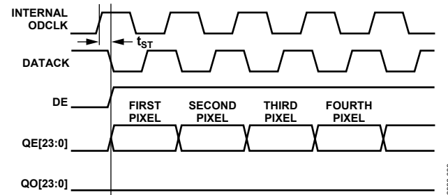
Figure 38. One Pixel per Clock (DATAACK Not Inverted)
