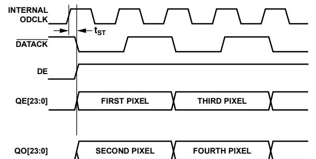
Figure 40. Two Pixels per Clock (DATAACK Inverted)
