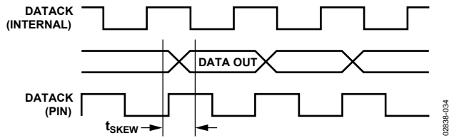
Figure 36. DVI Output Timing
