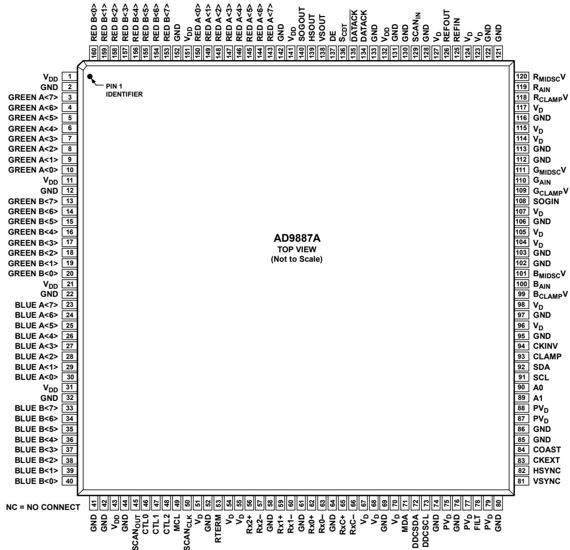
Figure 2. Pin Configuration
