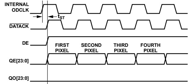
Figure 37. One Pixel per Clock (DATAACK Inverted)
