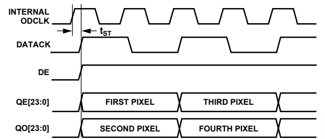
Figure 39. Two Pixels per Clock
