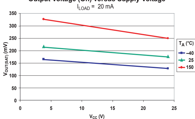
Output Voltage (On) versus Supply Voltage
