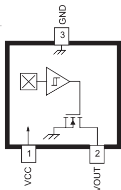
Package LH Pin-out Diagram
