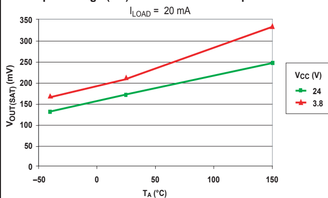
Output Voltage (On) versus Ambient Temperature
