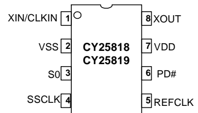
8-pin SOIC
