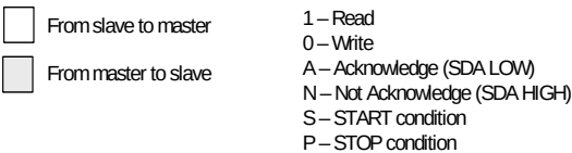
Figure 10. I 2 C Read Operation
