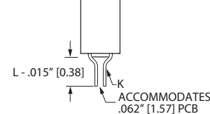
ACCOMMODATES .062" [1.57] PCB (CT, CS, CM, TK, CK, RS, RM) Example P/N: EBM10DCSN-S288 (Requires -S288 Modification Code)
