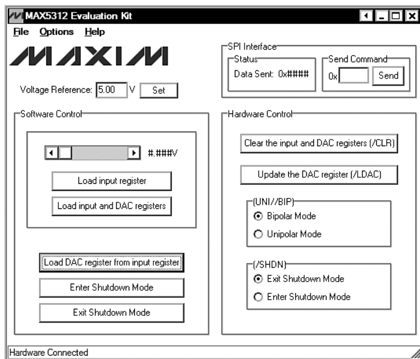
Figure 1. MAX5312 EV Kit Software Main Window
