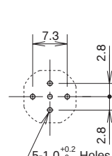
(PC Board Terminal Mounting Hole Layout)
