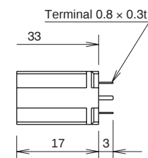
PC Board Terminal (AL-C1V)
