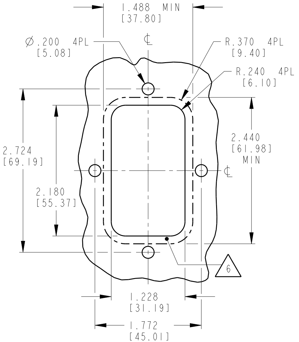
RECOMMENDED CUTOUT
