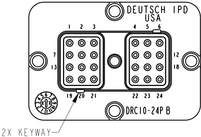
DRC10-24PB KEY -B-
