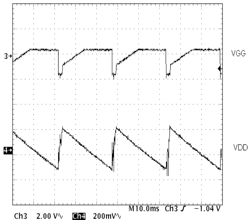
Figure 15. Ripple on VGG and VDD During Green Mode Operation
