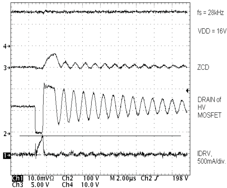
Figure 14. GM Mode Switching Cycle Waveform
