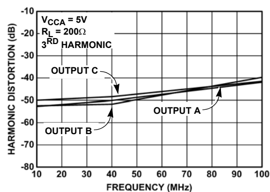
FIGURE 14. 3 RD HARMONIC DISTORTION
