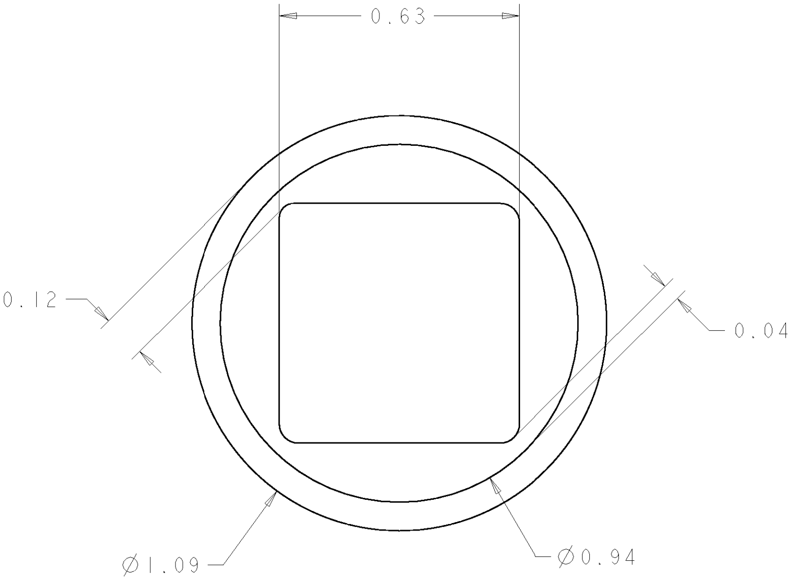
SOLDER TERMNIATION AREA SCALE 40:1
