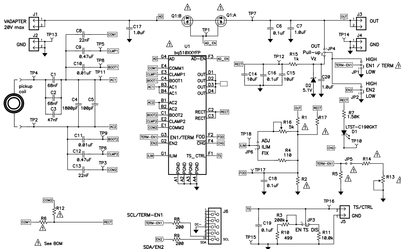
Figure 1. HPA764 Schematic
