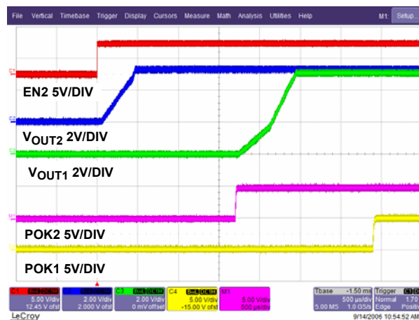
FIGURE 41. DELAYED START-UP ( V_{OUT1} = 5V , V_{OUT2} = 3.3V , EN1 = REF )
