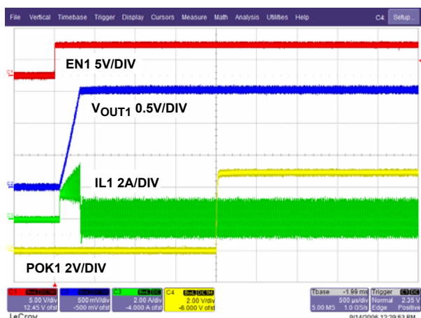
FIGURE 50. START-UP V_{OUT1} = 1.5V (NO LOAD, PWM MODE)S
