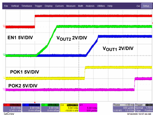
FIGURE 42. DELAYED START-UP ( V_{OUT1} = 5V , V_{OUT2} = 3.3V , EN2 = REF )
