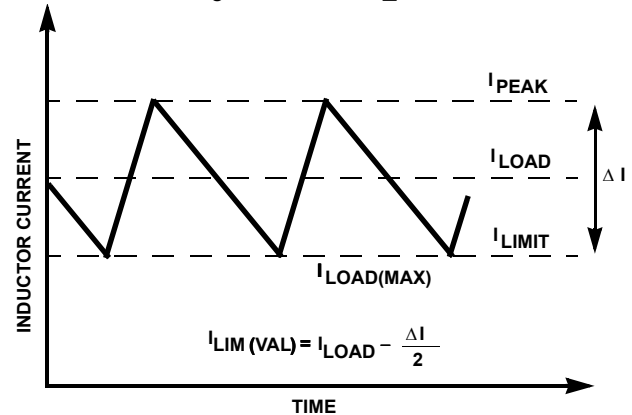
FIGURE 69. "VALLEY" CURRENT LIMIT THRESHOLD POINT
