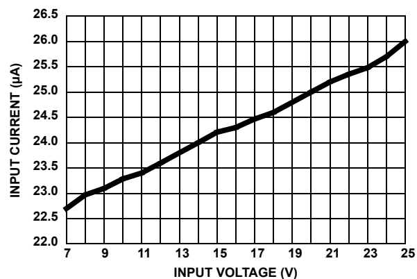
FIGURE 34. SHUTDOWN INPUT CURRENT vs V_{IN} ( EN = EN2 = EN\_LDO = 0 )
