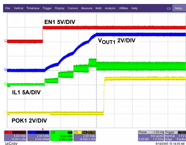
FIGURE 37. START-UP V_{OUT1} = 5V (FULL LOAD, PWM MODE)
