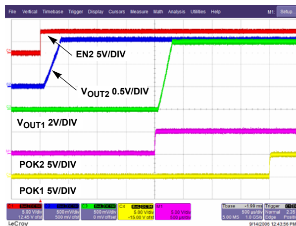
FIGURE 55. DELAYED START-UP ( V_{OUT1} = 1.5V , V_{OUT2} = 1.05V , EN1 = REF )
