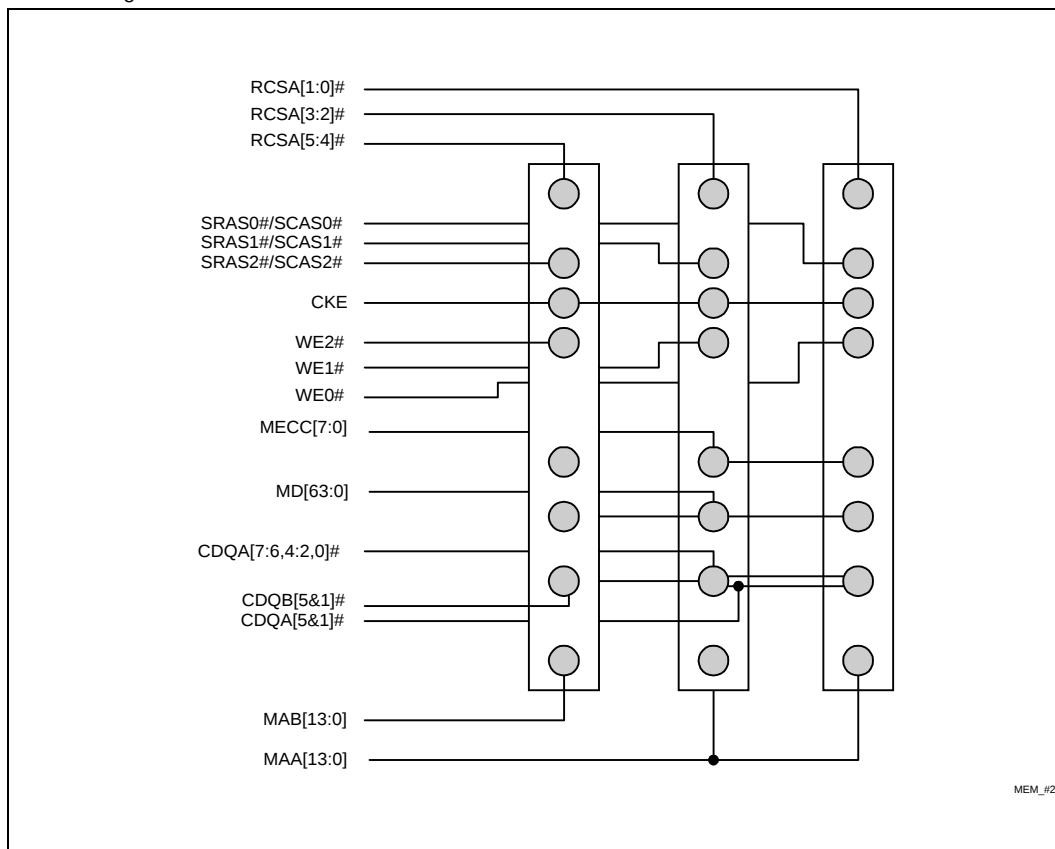
Figure 6. Configuration #2 (Small Memory Array)
