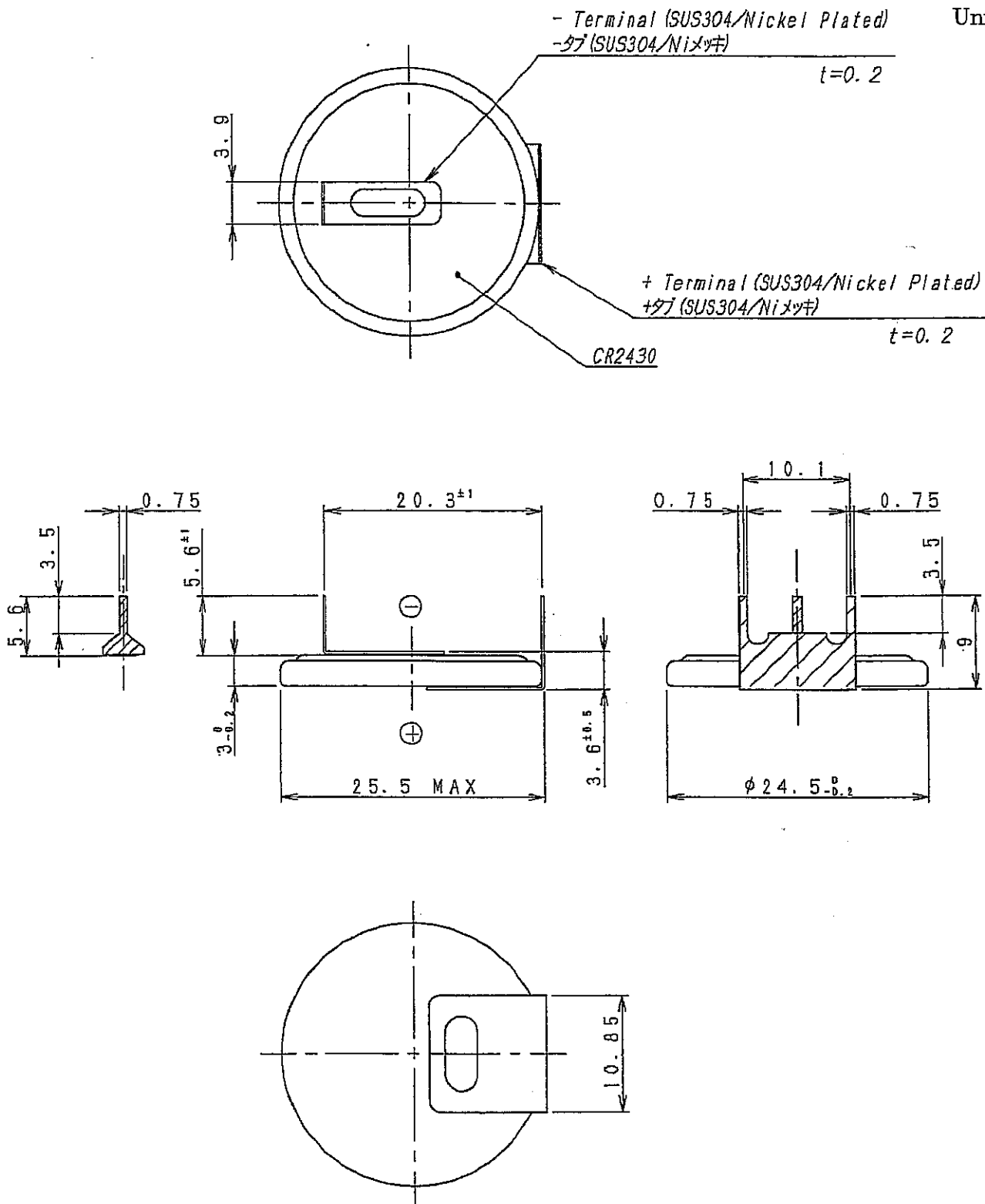
Fig.1 Shape and Dimensions Item : CR2430-F2ST7F
