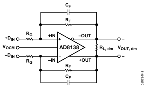
Figure 42. Circuit Definitions
