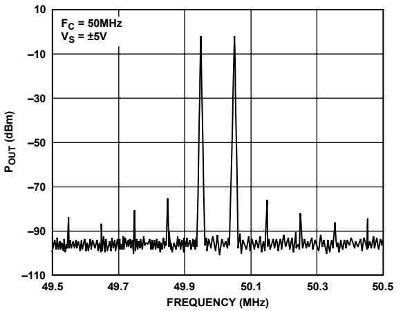
Figure 19. Intermodulation Distortion
