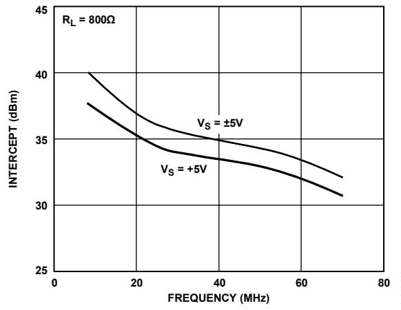
Figure 20. Third-Order Intercept vs. Frequency
