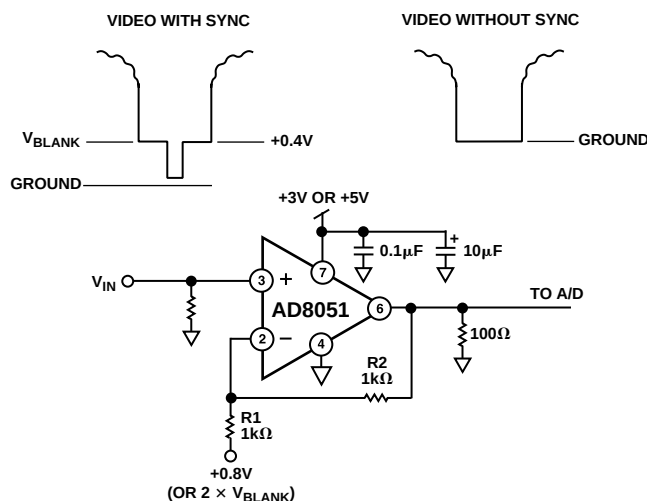
Figure 47. Sync Stripper
