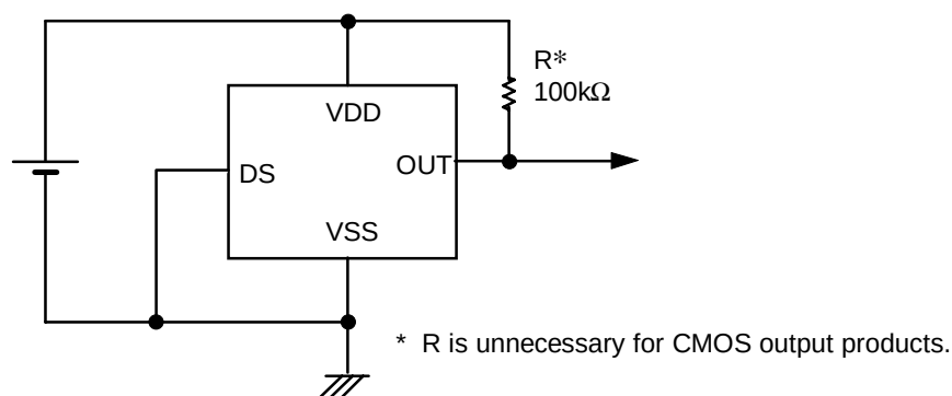
Figure 9 Standard Circuit
