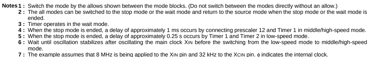
Fig. 62 State transitions of system clock
