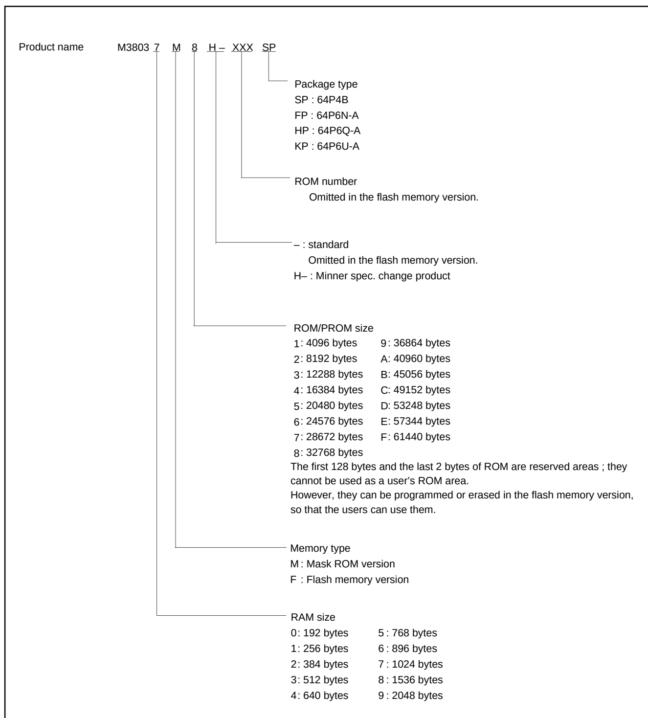
Fig. 4 Part numbering
