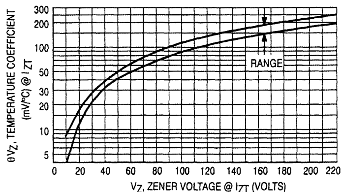
Figure 3. Temperature Coefficient-Range for Units 10 to 220 Volts
