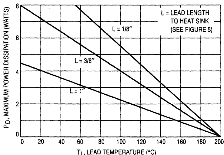
Figure 1. Power Temperature Derating Curve
