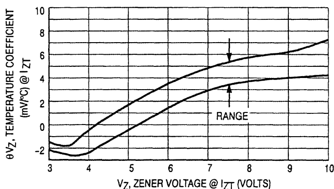
Figure 2. Temperature Coefficient-Range for Units 3 to 10 Volts
