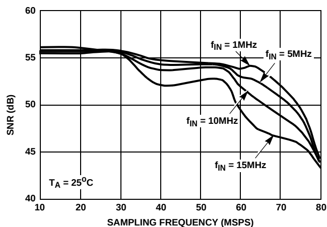
FIGURE 3. SNR vs SAMPLING FREQUENCY
