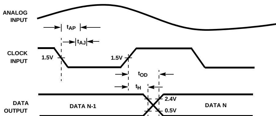
FIGURE 1. INPUT TO OUTPUT TIMING
