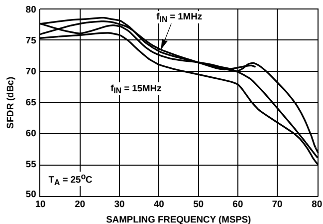
FIGURE 5. SFDR vs SAMPLING FREQUENCY
