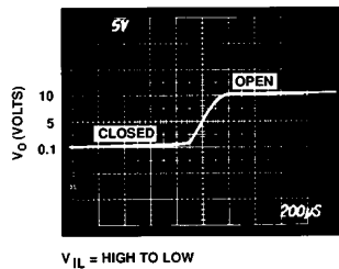
V_{IL} = \text{HIGH TO LOW}
