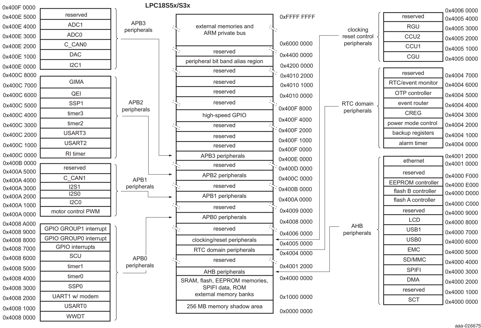
Fig 8. LPC18S5x/S3x Memory mapping (peripherals)
