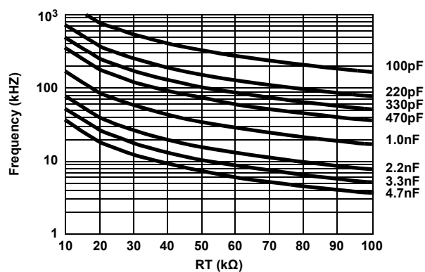
Figure 7. Resistance for CT Capacitor Values Given
