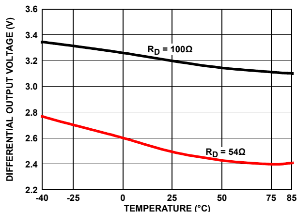
FIGURE 11. DRIVER DIFFERENTIAL OUTPUT VOLTAGE vs TEMPERATURE
