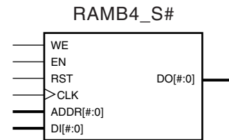
Figure 32: Single-Port Block SelectRAM+ Memory
